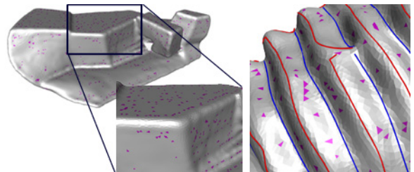
Figure 3: Singular triangles occur away from surface features. They are sparsely populated over the mesh. Illustrated for the lyon mesh (left) and a close-up of dino (right).
