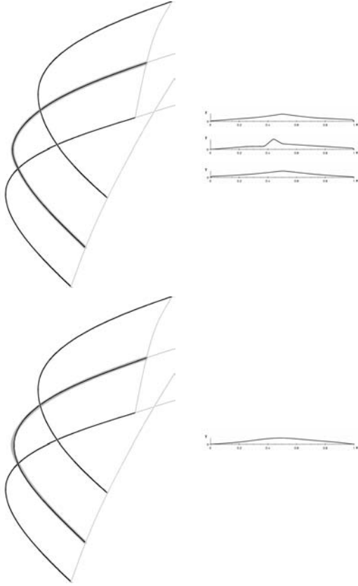
Figure 3. Smoothing of a curve of a patch layout. The curve in the middle has a bump, visible in the curvature plot. Smoothing removes the bump. The 3d \epsilon -constraint is shown in gray around the curve.
