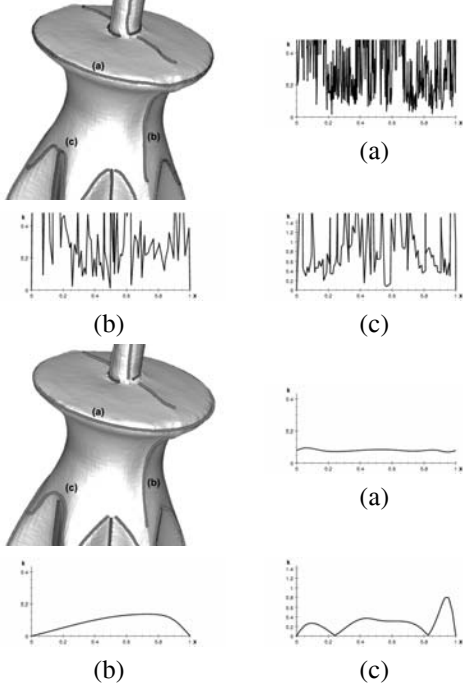
Figure 1. Feature lines on part of a screw driver, smoothed with the constraint CS-flow. Top row: The original lines created automatically by a feature detection algorithm [6] carry high frequency noise. Bottom row: CS-flow with \epsilon -constraint was used for the smoothing process to prohibit large deviations of the smoothed lines from the original surface. The plots show the scalar curvature |\kappa_c| of the curves.
